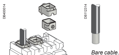
Bare cable.
