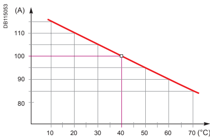
Temperature derating curve for CVS100.
