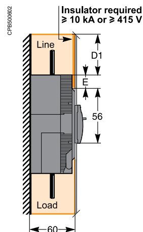
Minimal distance between the circuit breaker and front or rear panels
