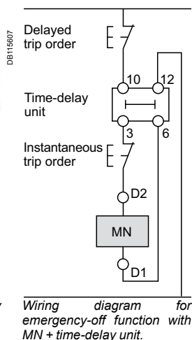
MN release with a time-delay unit.
